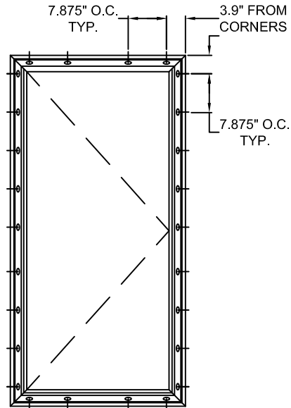
TYPICAL ELEVATION WITH FASTENER SPACING
